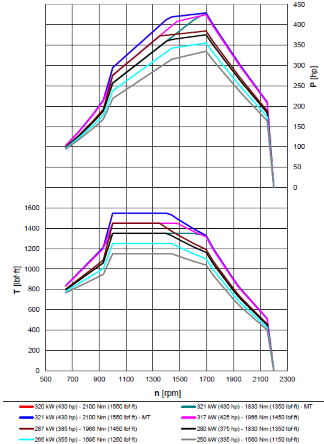
Graph 4.2 – MX-11 Power and Torque Curves
