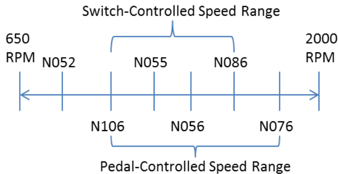
Figure 12.2 – PTO Engine Speed Limits and Set Points
