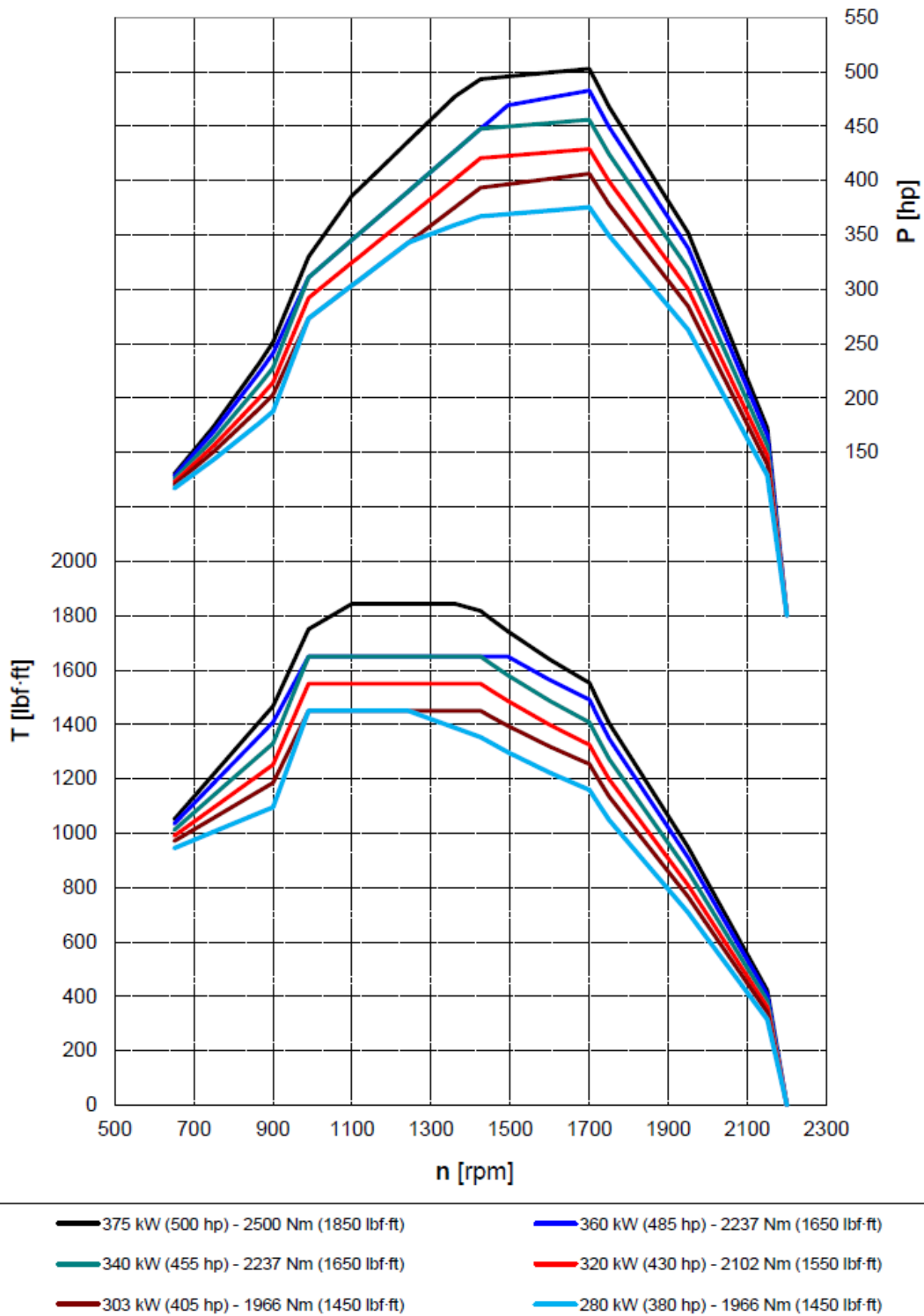
Graph 4.1 – MX-13 Power and Torque Curves
