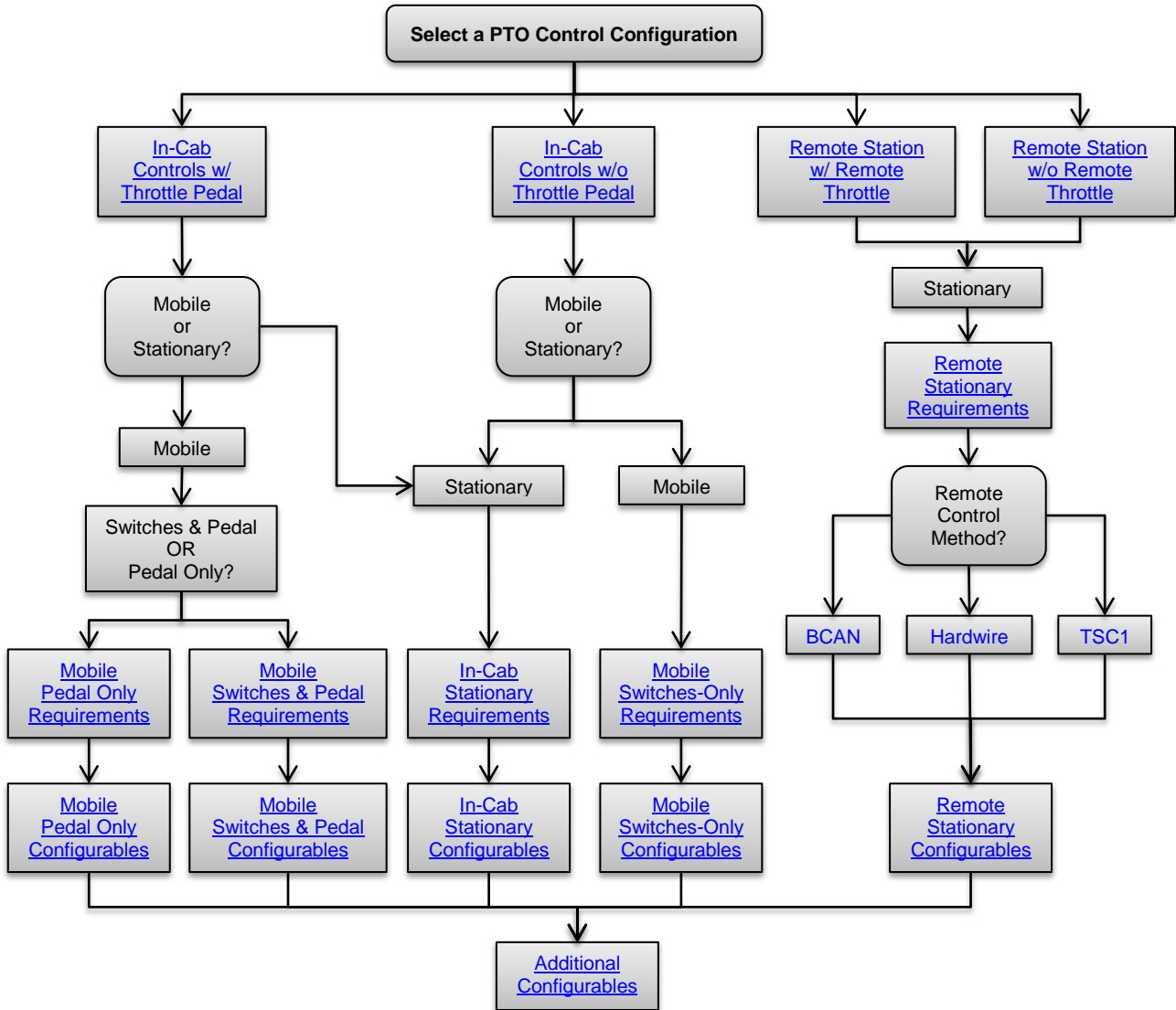
Figure 12.1 – PTO Control Configuration Flow Chart
